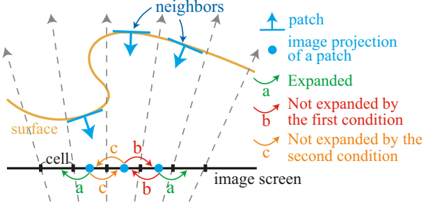
Fig. 5. (a) Given an existing patch, an expansion procedure is performed to generate new ones for the neighboring empty image cells in its visible images. The expansion procedure is not performed for an image cell (b) if there already exists a neighboring patch reconstructed there, or (c) if there is a depth discontinuity when viewed from the camera. See text for more details.
