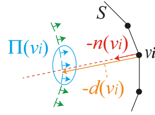
Fig. 8. In the iterative snapping algorithm, for each vertex \mathbf{v}_i on the mesh model, we first collect \pi (= 10) patches \Pi(\mathbf{v}_i) that are closest to the line defined by \mathbf{v}_i and a surface normal \mathbf{n}(\mathbf{v}_i) at the vertex. A (signed) distance d(\mathbf{v}_i) from \mathbf{v}_i to \Pi(\mathbf{v}_i) is used to compute photometric discrepancy term. See text for details.
