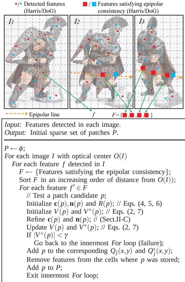
Fig. 4. Feature matching algorithm. Top: An example showing the features f' \in F satisfying the epipolar constraint in images I_2 and I_3 as they are matched to feature f in image I_1 (this is an illustration only, not showing actual detected features). Bottom: The matching algorithm.
