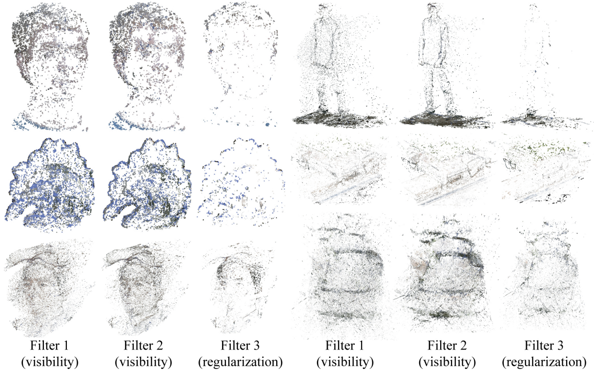
Fig. 13. Three filters are used to remove erroneous patches (Sect. III-C). The first two filters enforce global visibility consistency and the last filter enforces weak regularization. Patches detected as outliers by each of the three filters are shown for the first iteration of our algorithm. Note that more patches are added during the subsequent iterations, leading to the results of Fig. 11.
