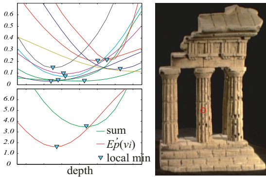
Fig. 9. Top left: Pairwise photometric discrepancy scores h(p, I_j) at a vertex of temple dataset. For better illustration, among three degrees of freedom in the optimization (a depth and a normal), the discrepancy scores are plotted for different values of depths with a fixed normal. A triangle on each plot illustrates the location of a local minimum, that is, a depth value obtained from the patch optimization procedure for a pair of images. Bottom left: The sum of all the pairwise discrepancy scores giving an inaccurate local minimum location, and our proposed photometric discrepancy energy (Eq. (11)). Right: an input image of temple with a red circle illustrating the location of the vertex.
