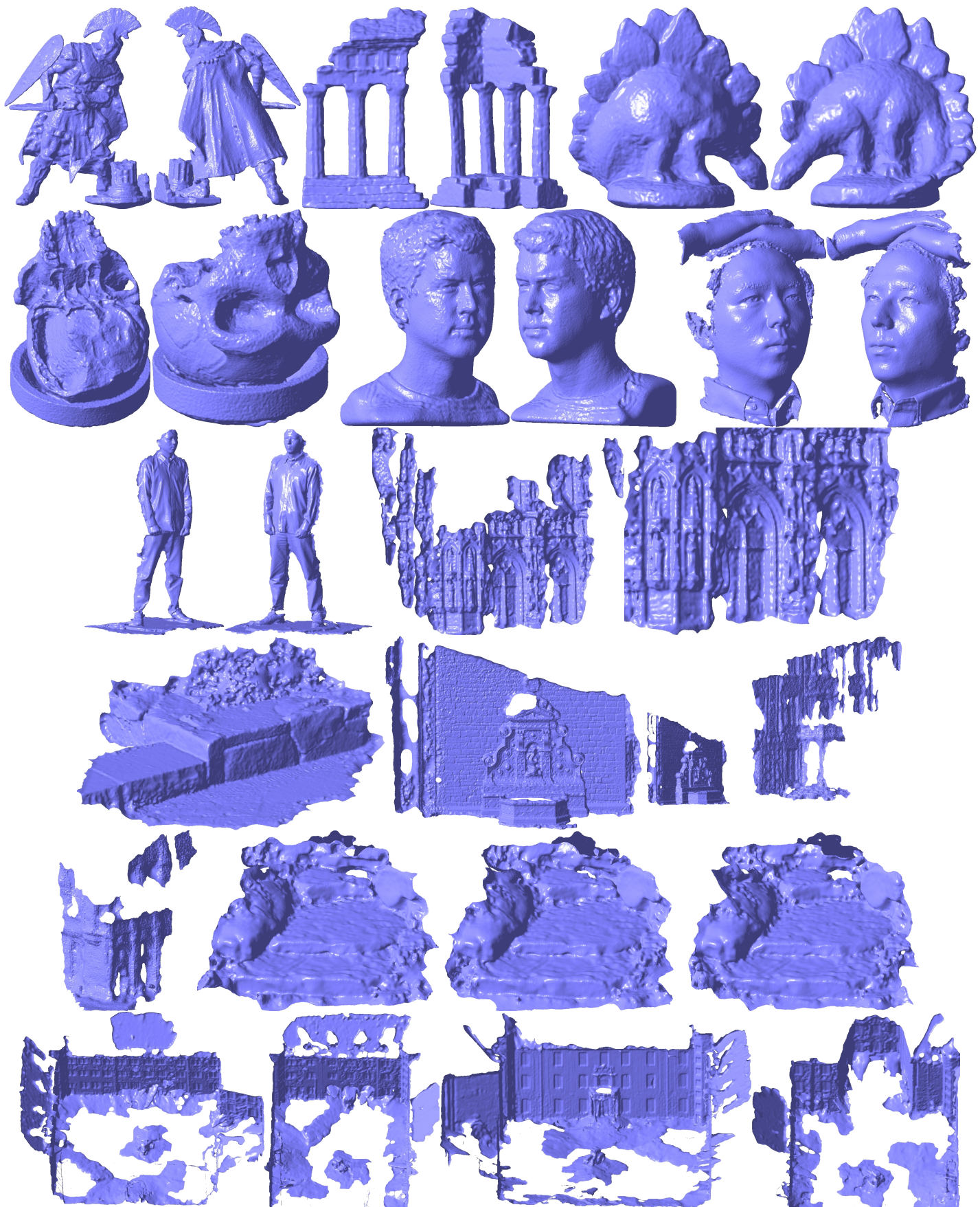
Fig. 16. Final mesh models: From left to right and top to bottom: roman , temple , dino , skull , face-1 , face-2 , body , city-hall , wall , fountain , brussels , steps-1 , steps-2 , steps-3 , and castle datasets. Note that the mesh models are rendered from multiple view points for fountain and castle datasets to show their overall structure.
