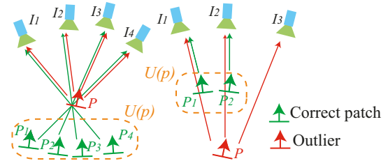
Fig. 7. The first filter enforces global visibility consistency to remove outliers (red patches). An arrow pointing from p_i to I_j represents a relationship I_j \in V(p_i) . In both cases (left and right), U(p) denotes a set of patches that is inconsistent in visibility information with p .
