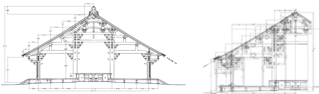
Figure 7 Drawings of Jodo-do, Jodo-ji
