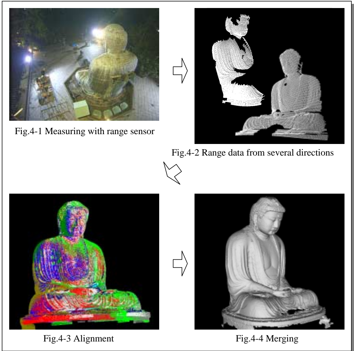
Figure 4 Modeling flow
