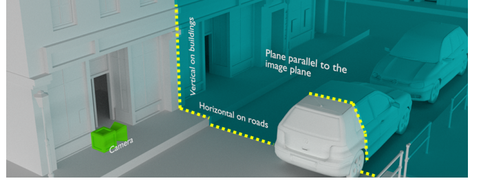
Fig. 3. The intersection between the plane parallel to the image plane and the 3D structures defines lines of which direction is dependent on the semantic class.
